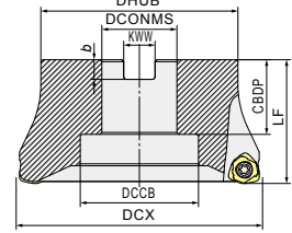
Fig.3 (エア穴無し) Without air hole
