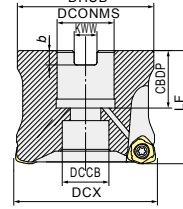
Fig.2 (エア穴付き) With air hole
