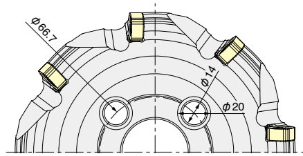
Fig.3 (エアーク無し) (Without air hole)
