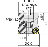
Fig.1 (エア穴付き) With air hole
