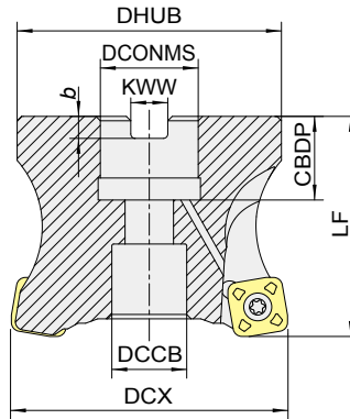
Fig.1 (エア穴付き) With air hole
